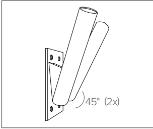
M36SS - Manchon mural double, incliné
